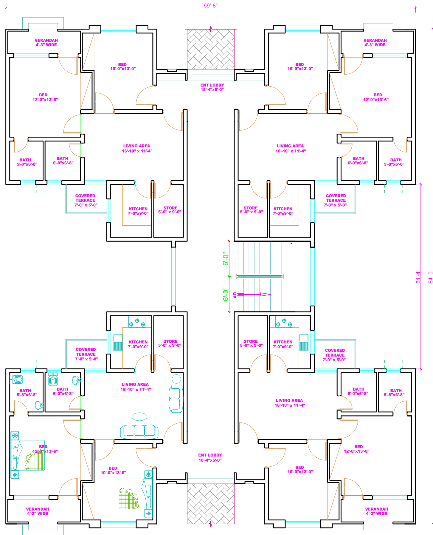
BLOCK PLAN
