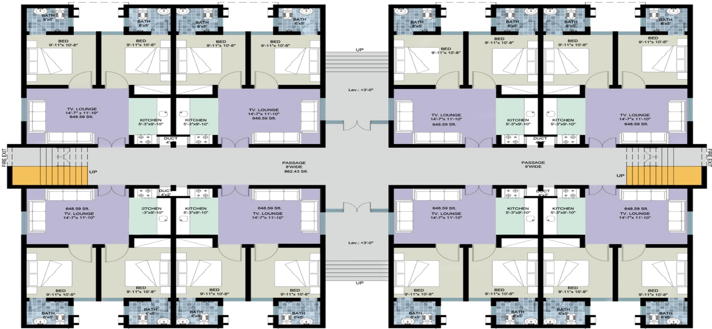
GROUND FLOOR PLAN WITH SHADE 6116.00 SFT. WITH OUT 6088.00 SFT.
